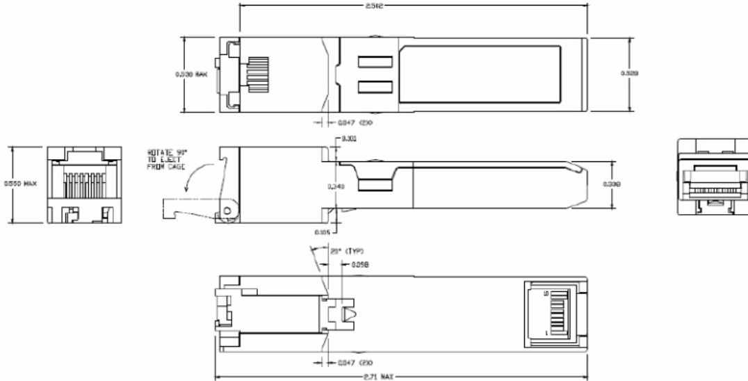
Figure2. Mechanical Specifications
