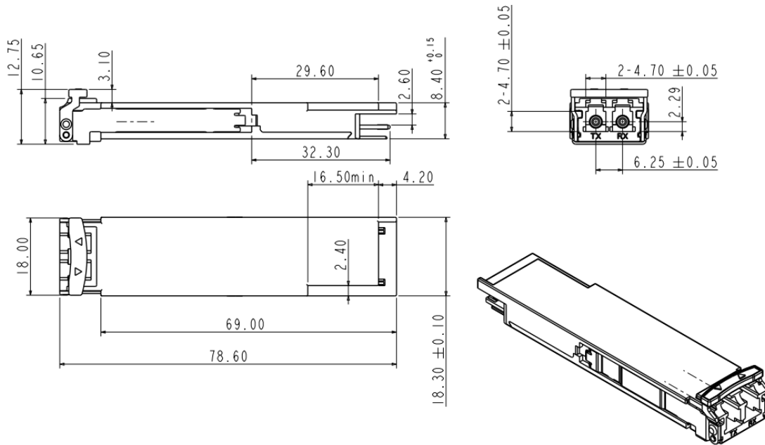
Figure4. Mechanical Specifications
