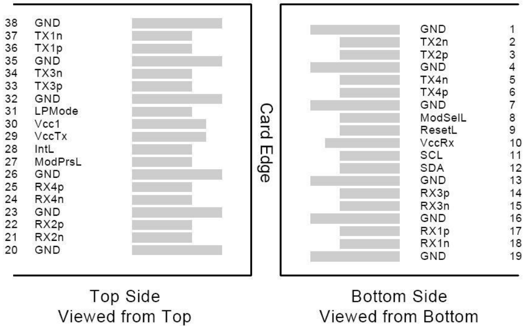
Figure3. QSFPE Edge Connector and Pinout Description
