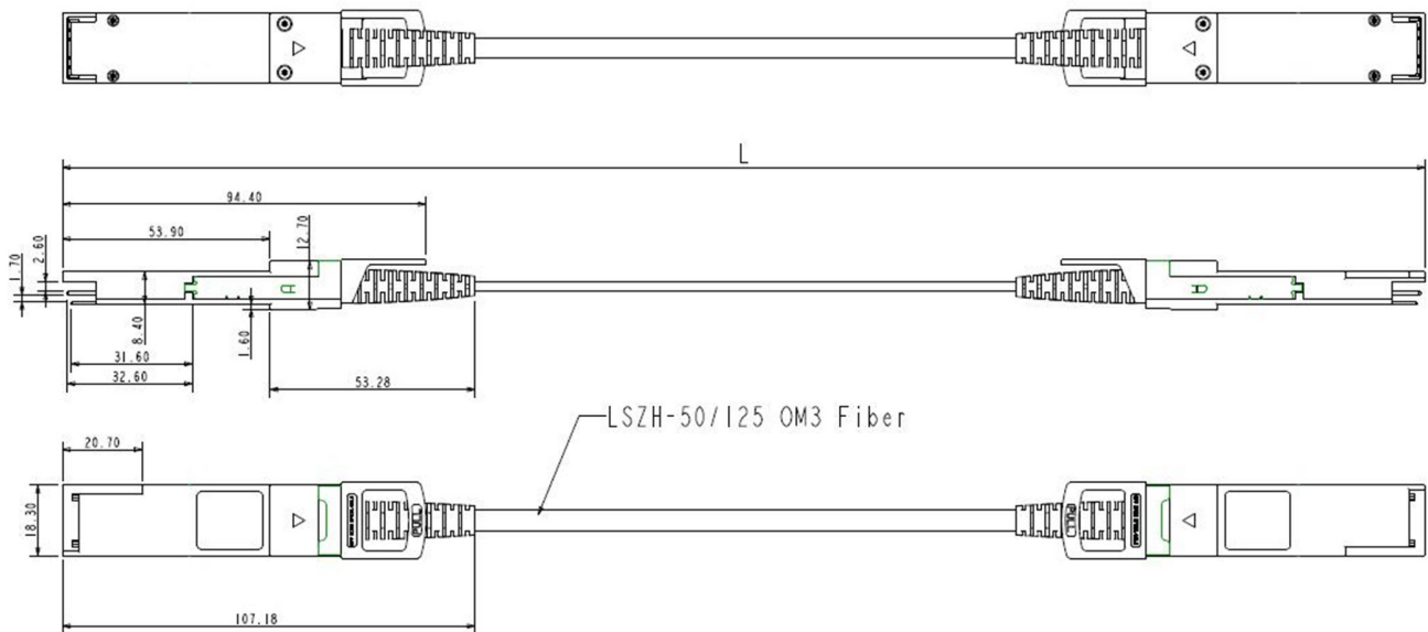
Figure2. Mechanical Specifications
