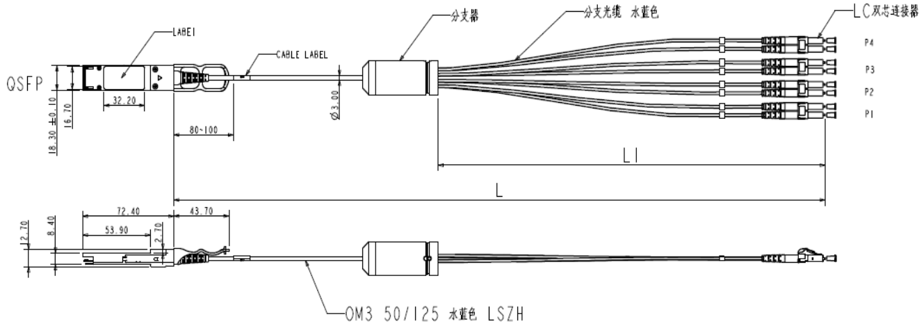
Figure2. Mechanical Specifications
