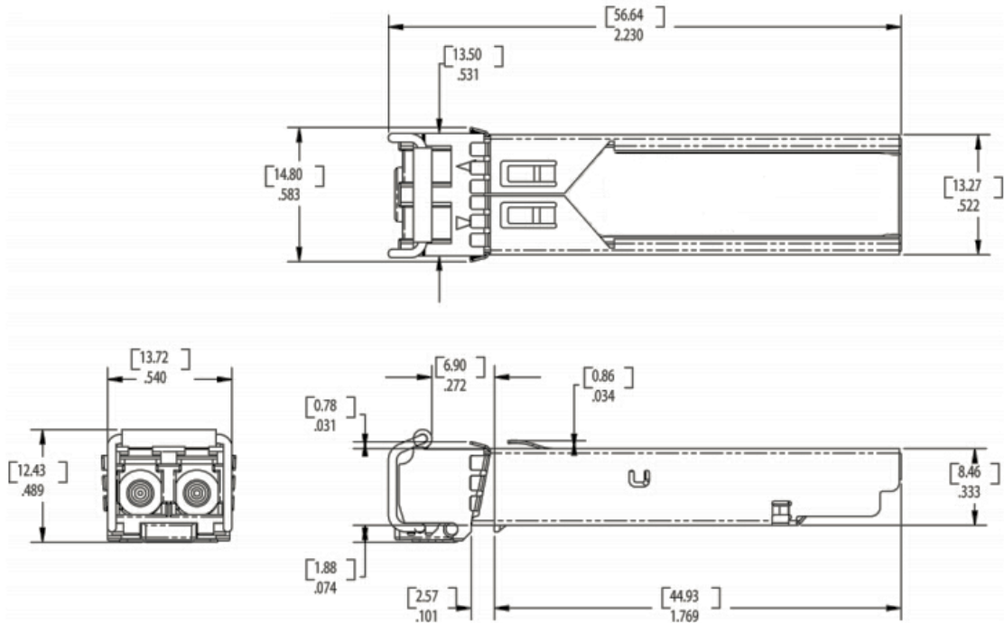
Figure5. Mechanical Dimensions
