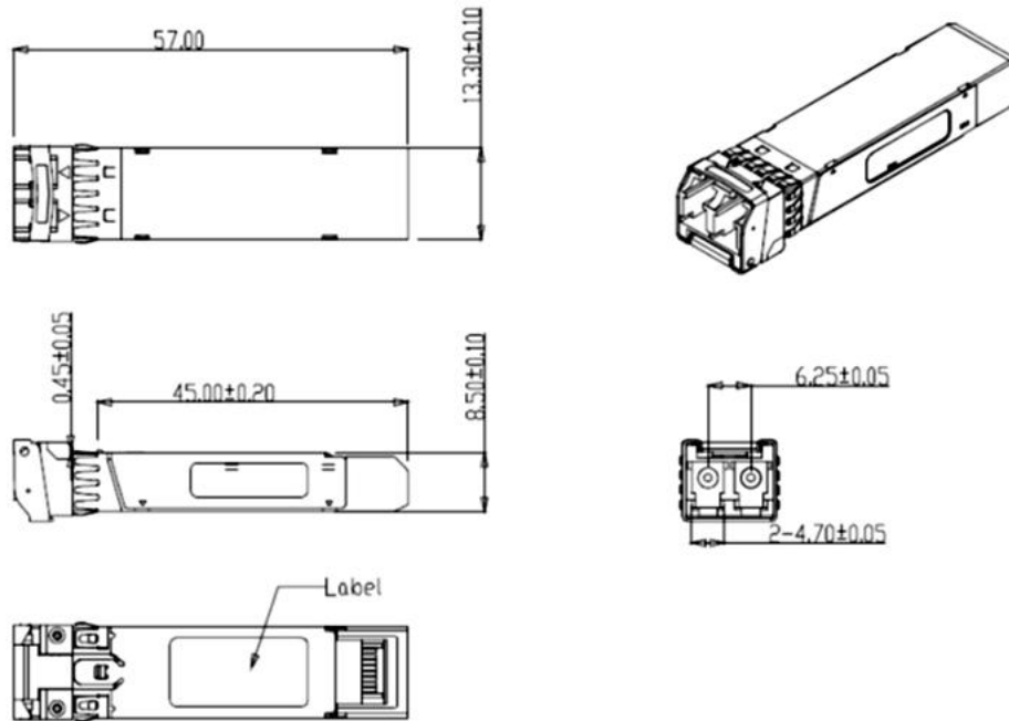
Figure5. Mechanical Specifications
